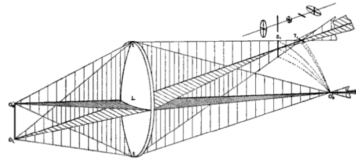
Figure 4.22: Astigmatism is primarily caused by incoming rays being off-axis in one plane, but close to perpendicular in another. (Figure from [361].)
