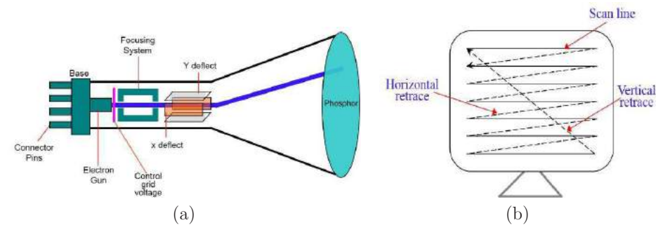
Figure 4.35: (a) In a cathode ray tube (CRT), an electron gun emits a beam of electrons, which are deflected in both X and Y directions according to an analog signal. When the beam hits the screen, an element of phosphor briefly lights up. (b) A special scanning pattern was used to draw out each video frame, line by line.
