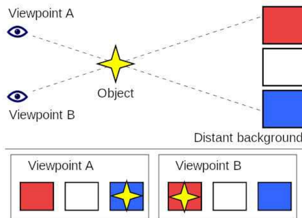
Figure 6.6: Motion parallax: As the perspective changes laterally, closer objects have larger image displacements than further objects. (Figure from Wikipedia.)
